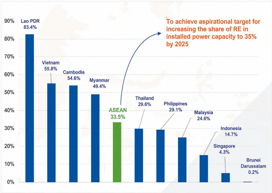
Fig. 10.2 Renewable Energy Share in ASEAN Member’s Installed Power Capacity 2020. Source: ASEAN Center for Energy (2022)
